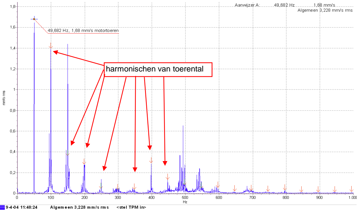
M 16 - MAZ - Verticaal - Snelh Freq 1000 Hz 9-4-04 11:48:24
